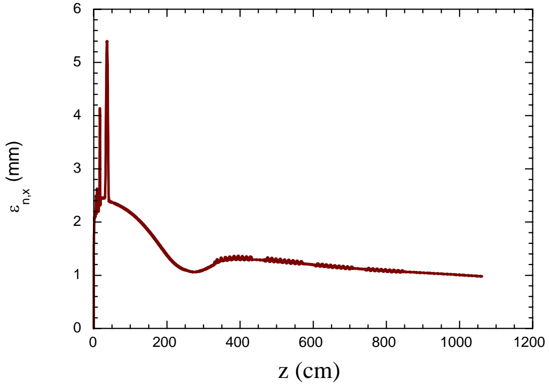
Figure 2. Rms normalized emittance evolution in SC photoinjector, from PARMELA simulations
