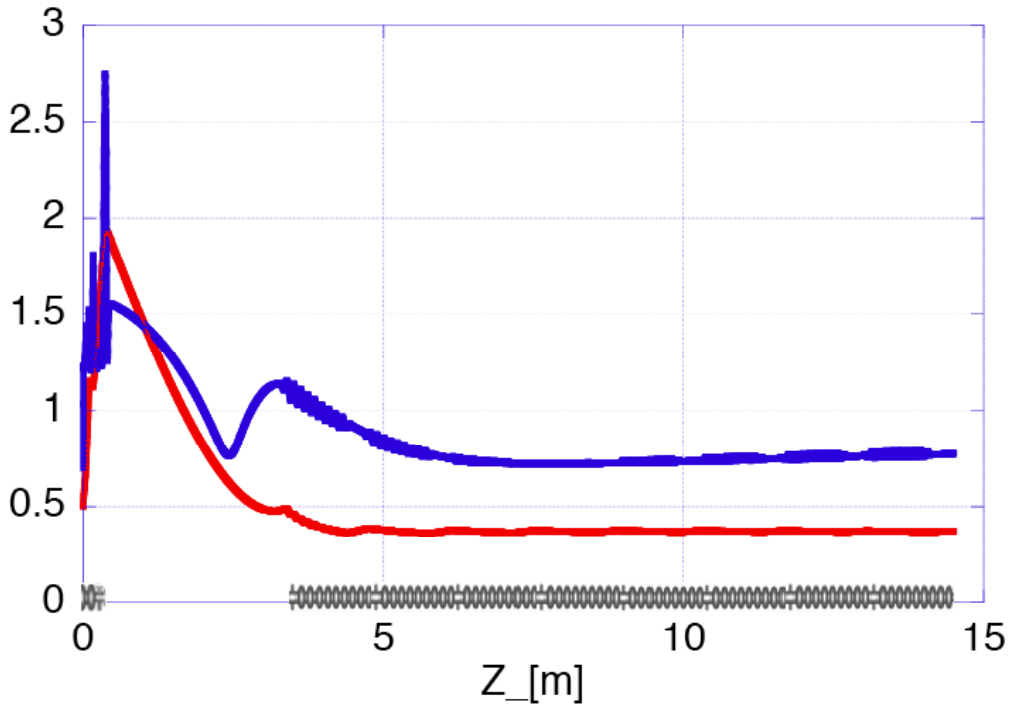
Figure 3. Rms normalized emittance [ \mu\text{m} ] (blue line) and beam envelope [mm] (red line) evolution along the SC photoinjector with reduced charge (0.35 nC) parameters, HOMDYN simulations
