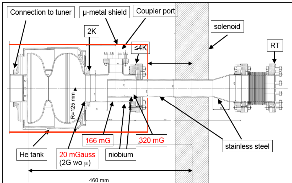
Figure 1 . Superconducting RF gun with coaxial input coupler and SC cathode, inside of cryostat assembly.
