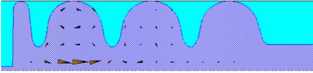
Figure 3: Profile of the magnetic field for the TE focusing mode as calculated with the MAFIA code.
