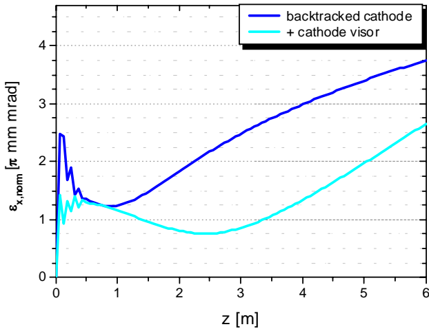
Figure 6: Normalized transverse emittance as calculated with the ASTRA code for the beam focusing with and without cathode visor.
