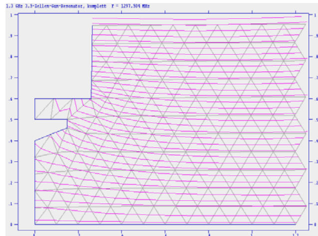
Figure 5: SUPERFISH sketch of the field lines near the retracted photocathode with visor.
