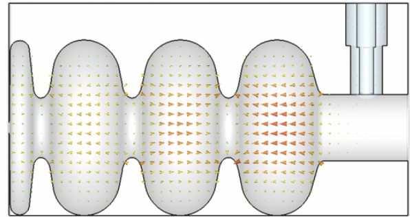
Figure 1: Profile of the electric field in the SCRF gun as calculated with the CST code.
