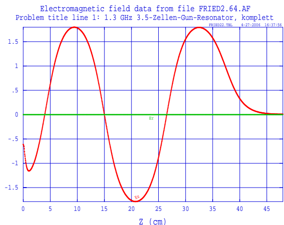
Figure 2: Distribution of the RF accelerating electrical field along the cavity axis as calculated with the Superfish code.
