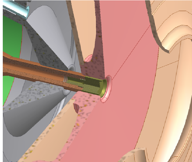
Figure 4: Retracted cathode with visor in the first half-cell of the SRF gun.
