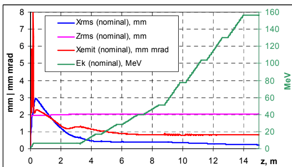
Figure 3: Electron beam parameters for the nominal setup: rms transverse size ( X_{rms} ), bunch length ( Z_{rms} ), normalized transverse projected emittance ( X_{emit} ). The mean kinetic energy ( E_k ) of the bunch is plotted on the right axis.
