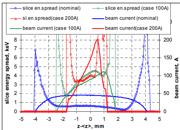
Figure 6: Slice energy spread and beam current profiles of electron bunch at z=15m .
