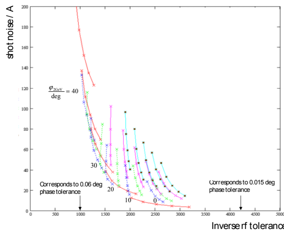
Figure 2: Shot noise in the undulator bunch profile (rms) and the inverse of the tightest rf tolerance for different bunch compression system working points. All points deliver a 5kA bunch, employing different rf phases and magnetic chicane strengths.
