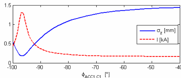
Figure 8: ASTRA [5] simulation of the rms bunch length and peak current the exit of ACC1 ( z=14.0 m ) versus the phase of the first cavity of ACC1.
